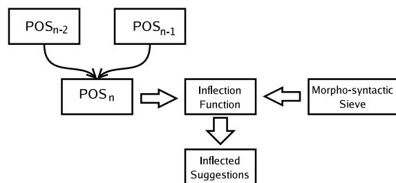
Figure 3. The Prediction Process of FastType.
