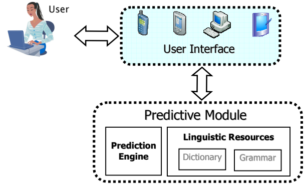
Figure 1. FastType Architecture.
